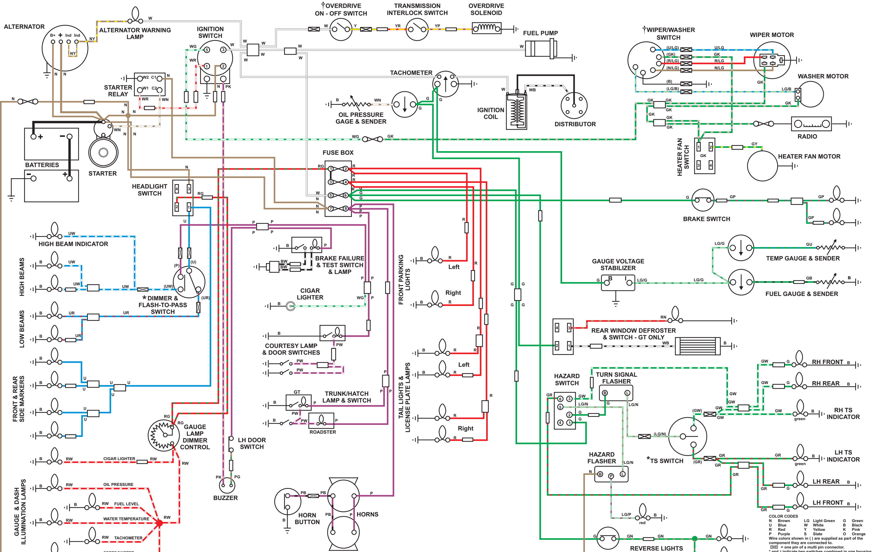
DIAGRAM 10 - 70/71 MGB FROM BENTLEY E3211W
