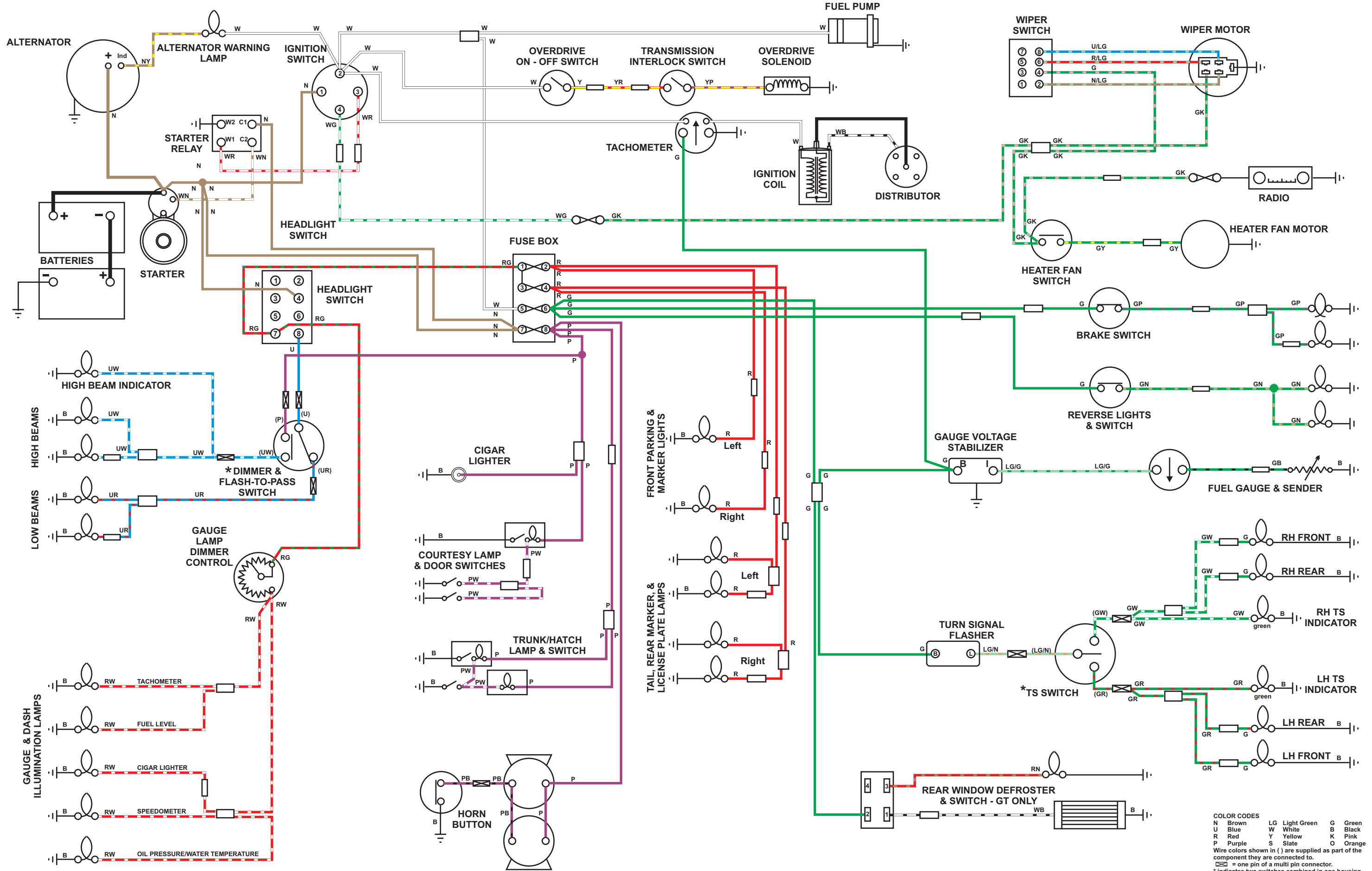
DIAGRAM 11 - 71/72 MGB FROM BENTLEY E3212AW
